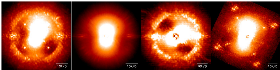
Figure 6.1: Coronagraphic focal plane images showing the asymmetry of the wind driven halo. Left: One exposure obtained with SPHERE-IRDIS (H2 band, 1.593 \mu\text{m} , \Delta\lambda \approx 53 \text{ nm} ). Middle left: One exposure obtained with SPHERE-IFS (second channel of YH mode, 0.991 \mu\text{m} , \Delta\lambda \approx 30 \text{ nm} ). Middle right: One exposure obtained with SPHERE-IRDIS in broadband (H band, 1.625 \mu\text{m} , \Delta\lambda \approx 291 \text{ nm} ). Right: One exposure obtained with GPI (second channel of YH mode, 1.503 \mu\text{m} , \Delta\lambda \approx 45 \text{ nm} ). The images are purposely stretched in intensity to highlight the asymmetry (log scale).
