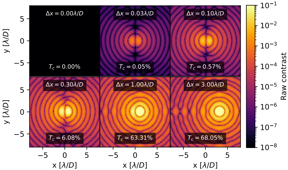
Figure 1.8: Images for on- and off-axis point sources through a second-order perfect coronagraph. For each image, the core throughput, the fraction of light inside a 1.4\lambda/D diameter circle centered on the object, is listed.
