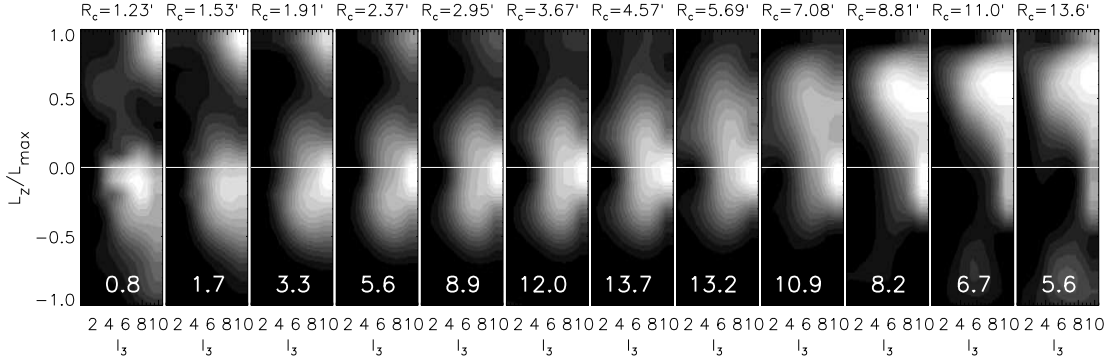
FIGURE 19 — The orbital weight distribution for our best-fit model of \omega Cen. From left to right, the panels show the orbital weight distribution at increasing distance from the center, which corresponds to increasing energy. The radius R_c (in arcmin) of the circular orbit at the corresponding energy is given above each panel. The radial range that is shown is constrained by the observations and contains more than 90% of the total cluster mass. The vertical axis represents the angular momentum L_z in units of L_{\max} , the angular momentum of the circular orbit. The horizontal axis represents the third integral I_3 , parameterized by the number of the (linearly sampled) starting angle of the orbit. Black shading corresponds to zero orbital weights, and white corresponds to the maximum orbital weight in each panel. At the bottom of each panel the fraction (in %) of the included mass with respect to the total mass is indicated. (See p. 250 for a color version of this figure.)
